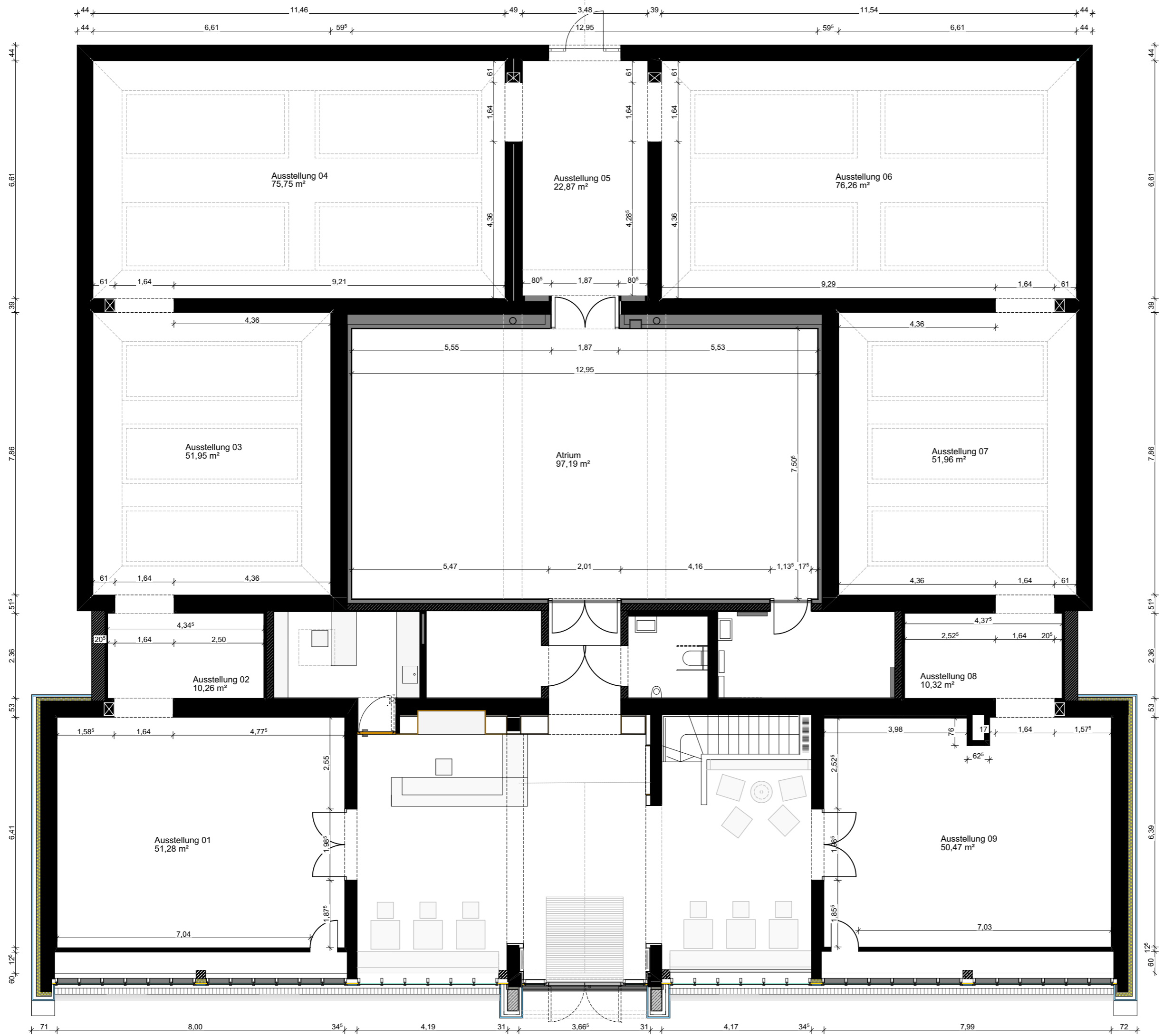
Kallmann Museum Ismaning Grundriss M 1:100 A3
